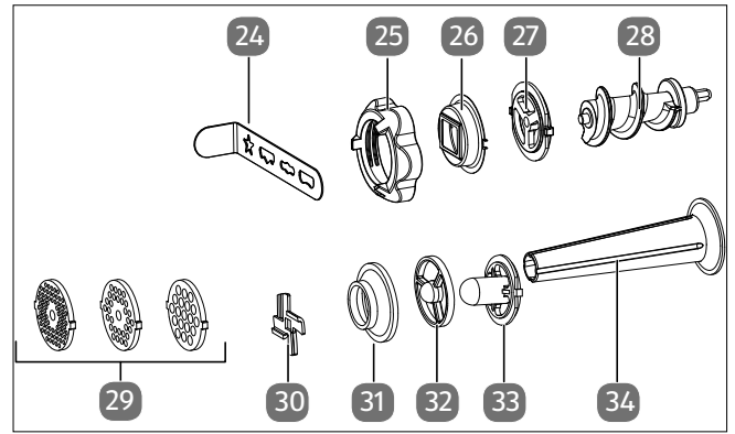
Fig. 6 – Mincer accessories
