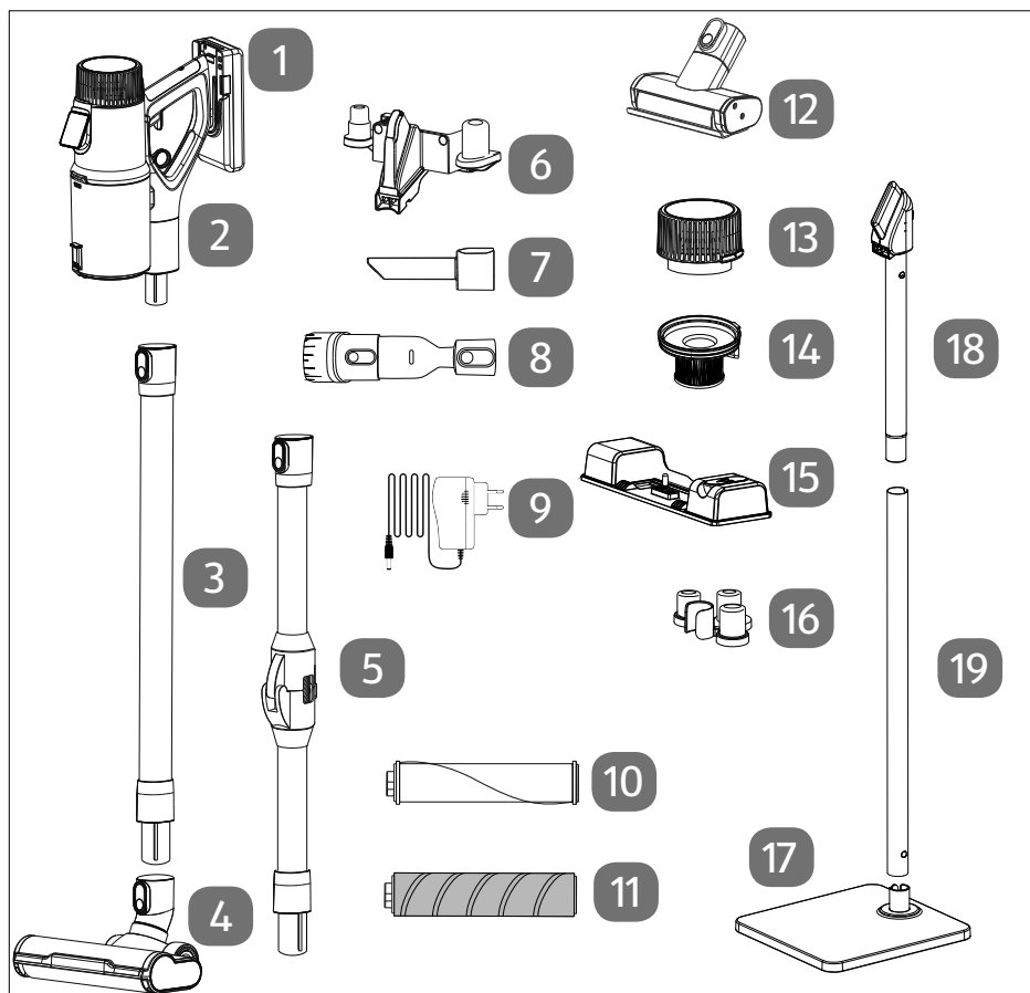
Fig. 1 – Appliance overview and accessories
