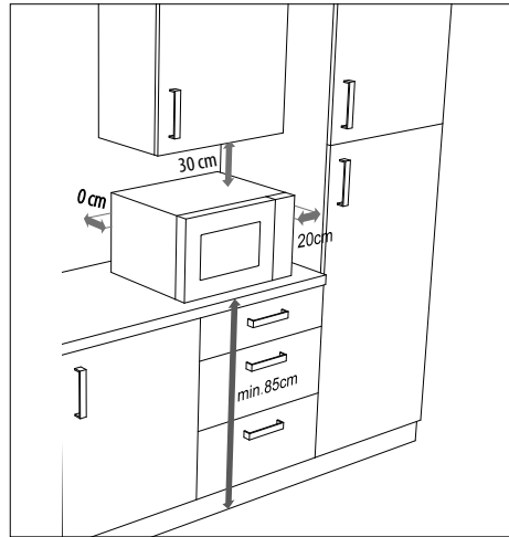
Abb. 2 – Appliance clearance
