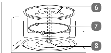
Abb. 3 – Inserting the glass turntable
